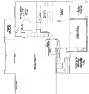
1 MAIN FLOOR PLAN SCALE: 1/8" = 1'-0"
