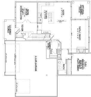
1 MAIN FLOOR PLAN SCALE: 1/8" = 1'-0"
